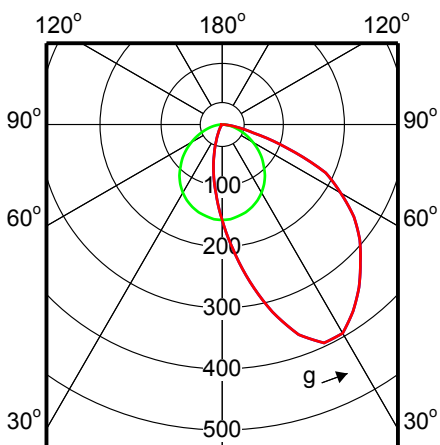
(cd/1000lm) 0° L.O.R.=0.60 — 0-180° — 90-270° TBS105 1xTL-D58W HFP A
