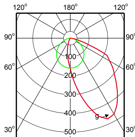
(cd/1000lm) 0° L.O.R.=0.67 — 0-180° — 90-270° TBS105 1xTL5-35W HFP A
