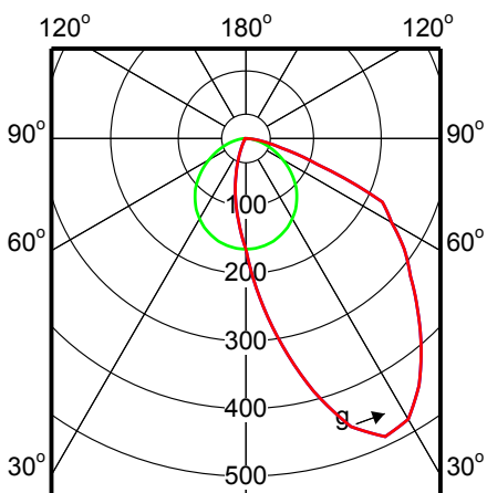
(cd/1000lm) 0° L.O.R.=0.69 — 0-180° — 90-270° TBS105 1xTL5-49W HFP A
