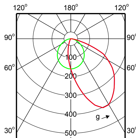
(cd/1000lm) 0° L.O.R.=0.61 — 0-180° — 90-270° TBS105 1xTL-D36W HFP A
