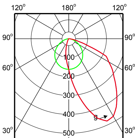
(cd/1000lm) 0° L.O.R.=0.68 — 0-180° — 90-270° TBS105 1xTL5-54W HFP A
