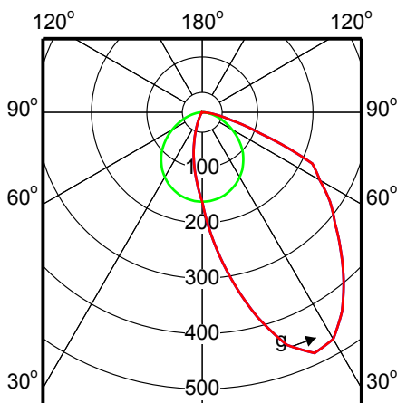
(cd/1000lm) 0° L.O.R.=0.68 — 0-180° — 90-270° TBS105 1xTL5-28W HFP A
